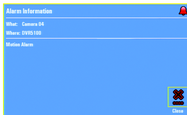
Figure 42. Alarm Information
